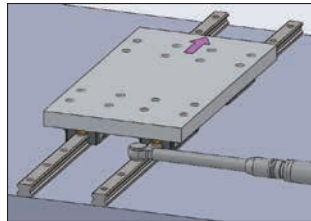
Fig 1.11.16 Compare to the master Linear Guide rail
